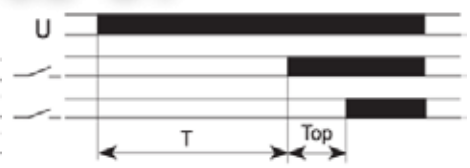
FZ31: Symmetrical recycling, OFF start, with signal contact
