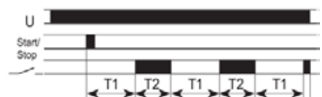
FZ40: Symmetrical recycling, OFF start with Start/Stop pushbutton
